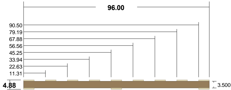
Side View
