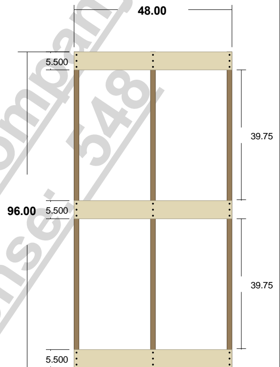
Bottom View
